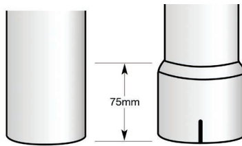
Plain End Expanded & Notched End Plain End Expanded & Notched End
