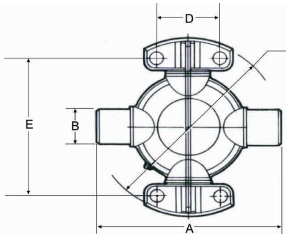
LWD – Low Wing Drilled LWT – Low Wing Threaded
