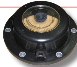
Trailer 6-1/4" OD 1-5/8" Deep 1613 Bolt Holes 5-1/2" Circle Replaces Steel 1703
