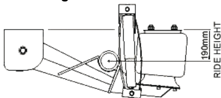
Underslung
