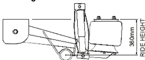
Overslung
